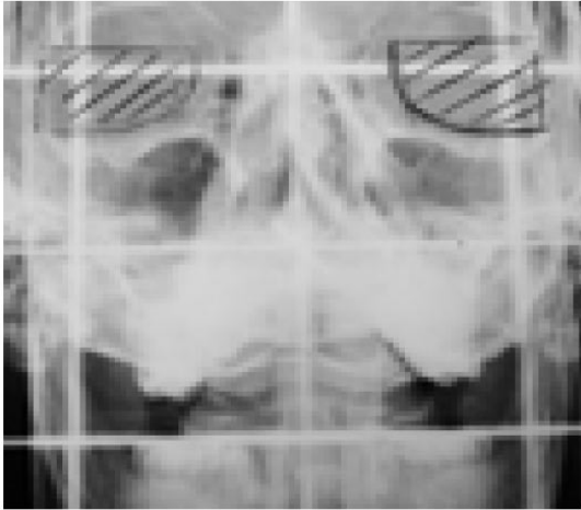
Figure 24 : Champ nasal
