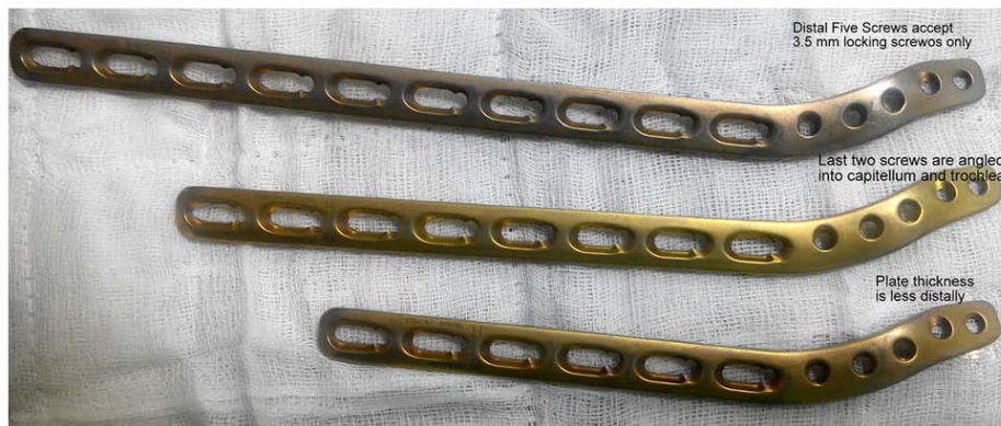
Figure n35 Plaque LCP , pré contournée
