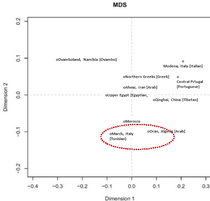
Figure 9. Multidimensional Scale (MDS) representation of 17Y-STRs in a sample of Moroccan population (Arabic, Berber and Sahrawi) and other Middle Eastern and Mediterranean populations [20].
