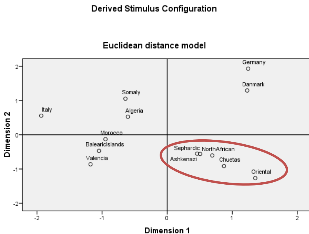
Figure 22: Multidimensional scaling analysis (MDS) based on pairwise genetic distances calculated between 13 populations for 12 X-STRs. Stress: 0.18645 RSQ= 0.81648
