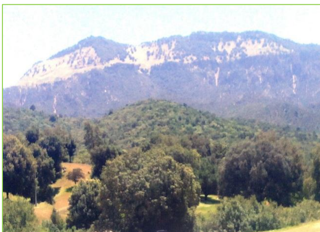
Photo 65: Anticlinal-faillé, Jbel Boutarwa
