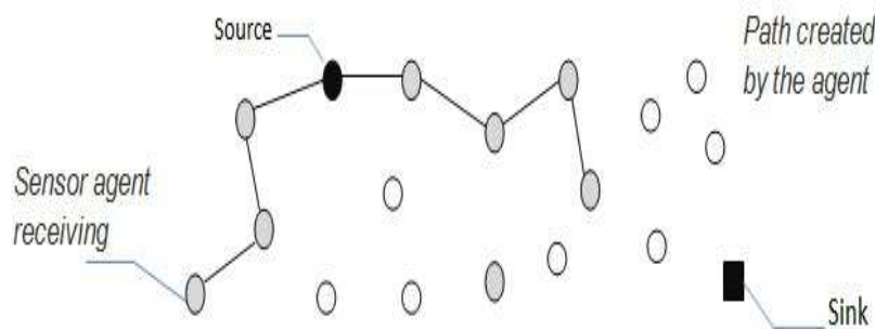
FIGURE 2.27 – Agents events
