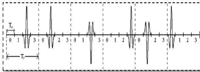
FIGURE 2.12 – radio pulses generated by UWB
