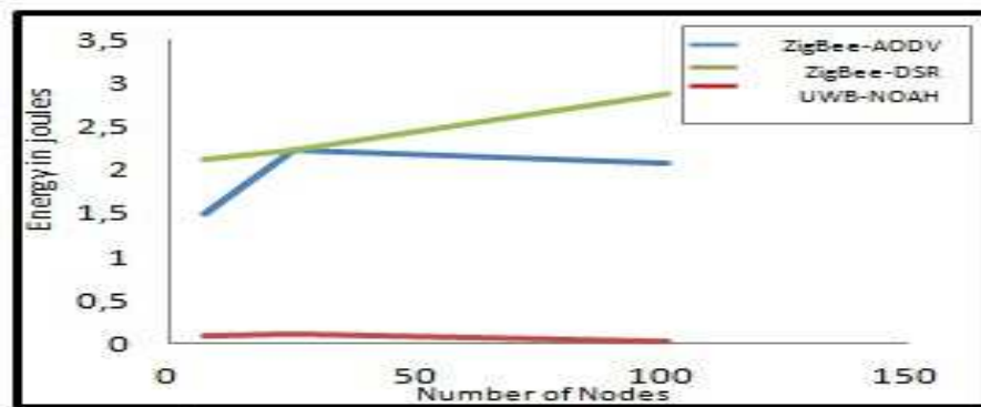
FIGURE 3.12 – Energy Consumption
