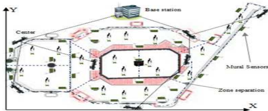
FIGURE 3.36 – Sample of mural sensors deployment and zone repartition.
