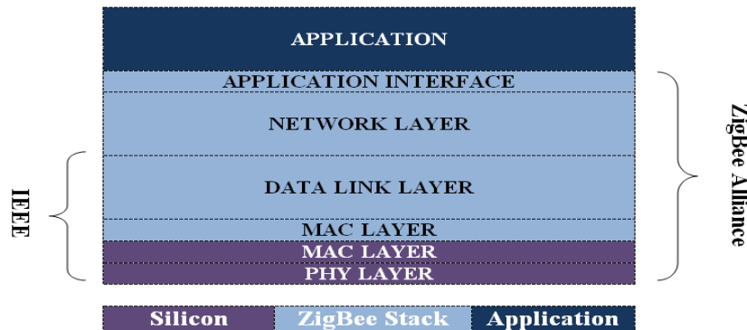
FIGURE 2.11 – Protocol stack of ZigBee (IEEE 802.15.4a)
