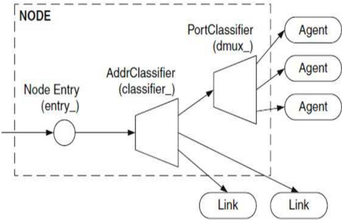
FIGURE A.2 – Node Architecture in NS2
