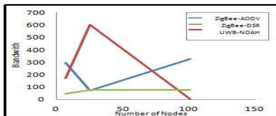
FIGURE 3.10 – Bandwidth
