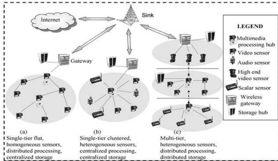
FIGURE 2.6 – WMSN Architecture
