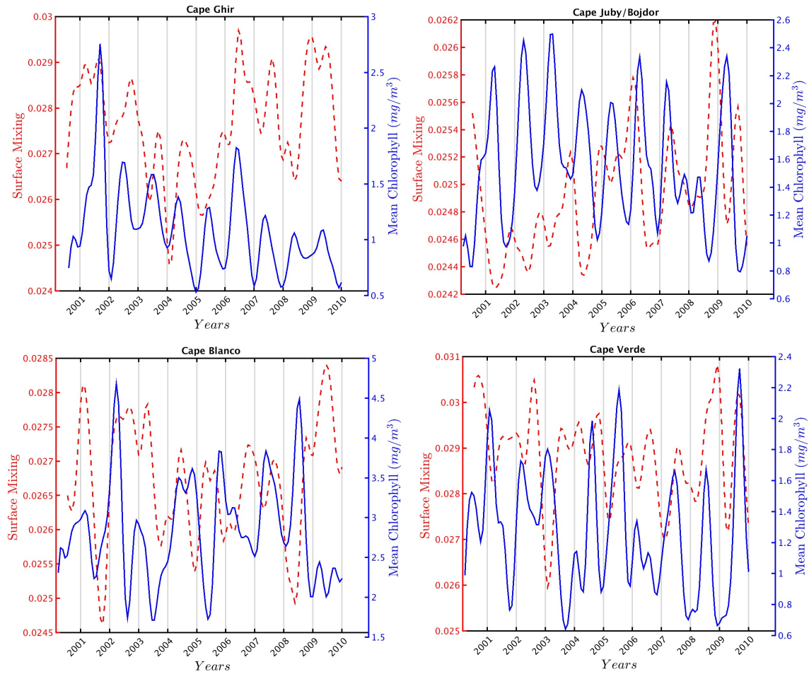
Figure 5-4: Interannual variation of the surface mixing versus the fronts chlorophyll concentrations. Red axis for the mexing and the blue one is for the cholorophyll concentrations (monthly-mean).
