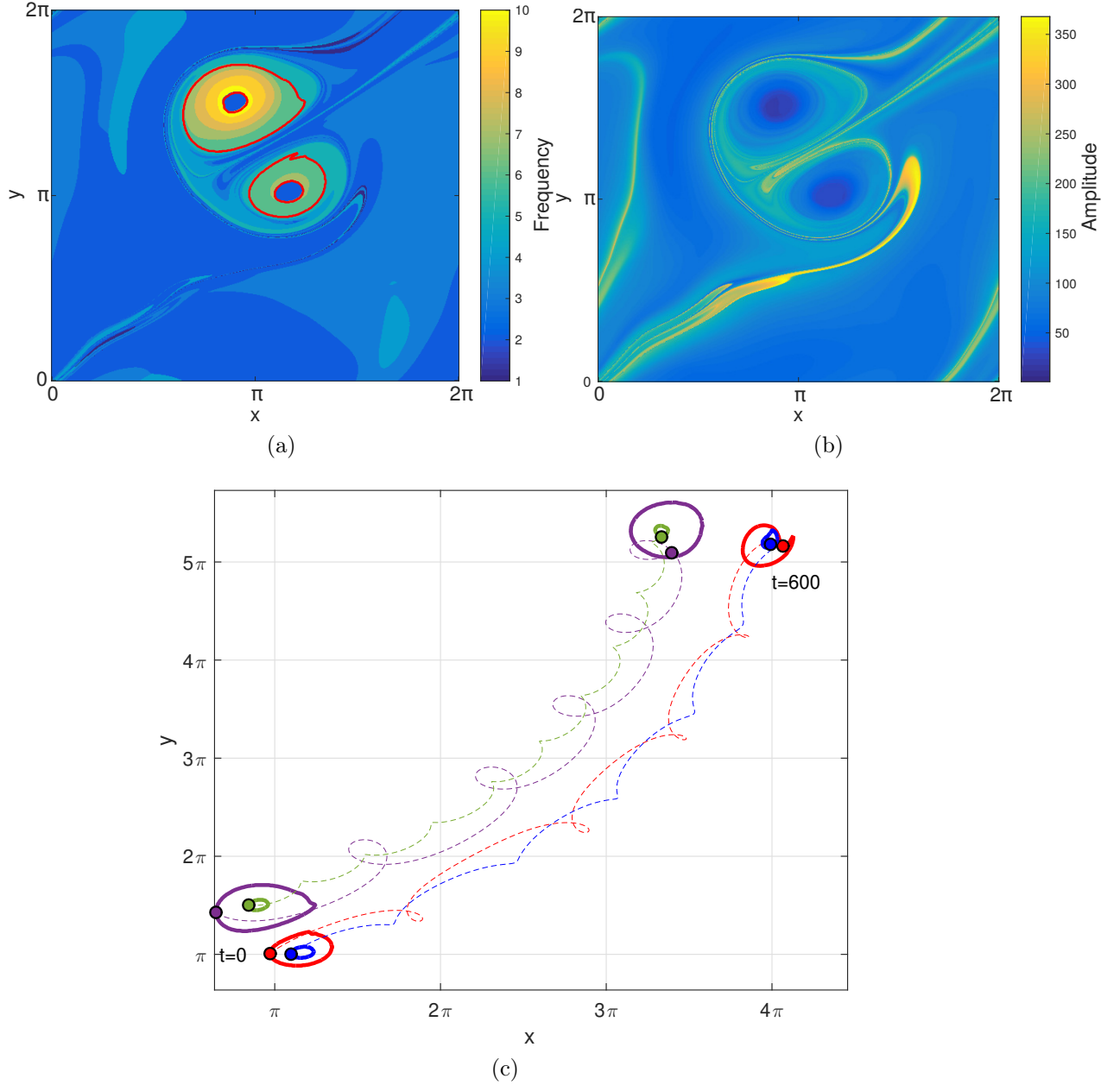
Figure 7-6: a) Lagrangian coherent vortices at time t_0 extracted from the velocity field generated by Navier-Stokes model 7.10 using definition.1 with the \bar{\xi} map shown in background, with \xi \mapsto |\mathcal{LTF}^\xi(\mathbf{x}_0)|^2 . b) The mean-average magnitude |\mathcal{LTF}^\xi(\mathbf{x}_0)| highlighting areas of spinning movement. c) Their initial and final positions under Lagrangian advection as well as different particles initialized within their boundaries and their trajectories in Dashed line. (See the supplemental movie M7 for the complete advection sequence of these vortices.)
