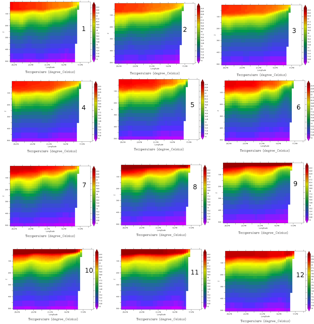
Figure 3-10: GLORYS2V4: monthly Temperature V-section of the year 2010 in the point (lat = 21.42°N lon = -18.51°N)
