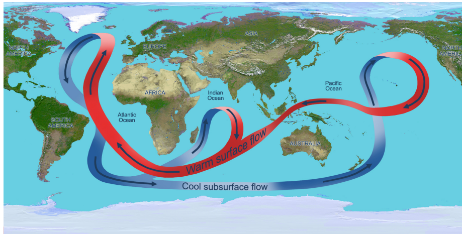
Figure 1-4: World's map showing the thermohaline circulation. Blue paths represent cool deep-water currents, while red paths represent warm surface currents 4 .
