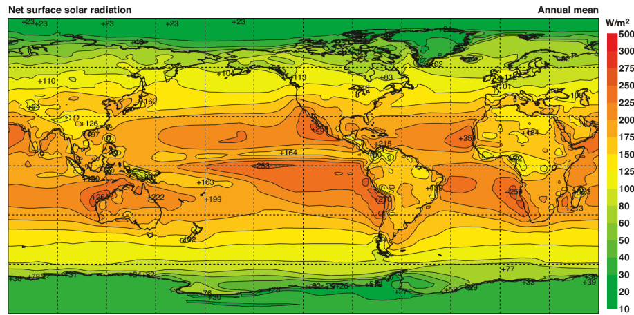
Figure 1-2: Heating of earth's surface by solar radiation, in \text{W/m}^2 , calculated from the ECMWF 40-year reanalysis of atmospheric data. The tropics absorb more heat than they lose, while the poles lose more heat than they absorb. This imbalance drives the planetary heat engine 2 .
