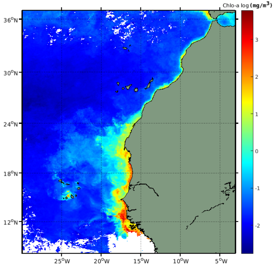
Figure 1-11: MODIS 30-day CHL a concentration image over the North-West African margin. Each pixel presents CHL a concentration in ( \log(mg/m^3) ). This image is obtained on the first week of January 2001 and it is showing a typical upwelling scenario over the studied area.
