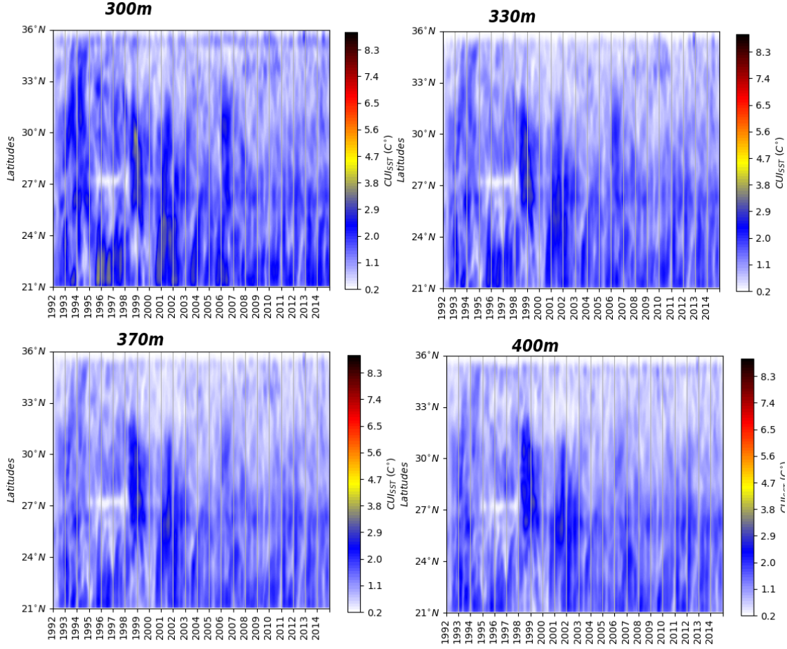
Figure 3-11: Space-time Hovmöller plot of the seasonal and interannual variability of the I^r at different depths.
