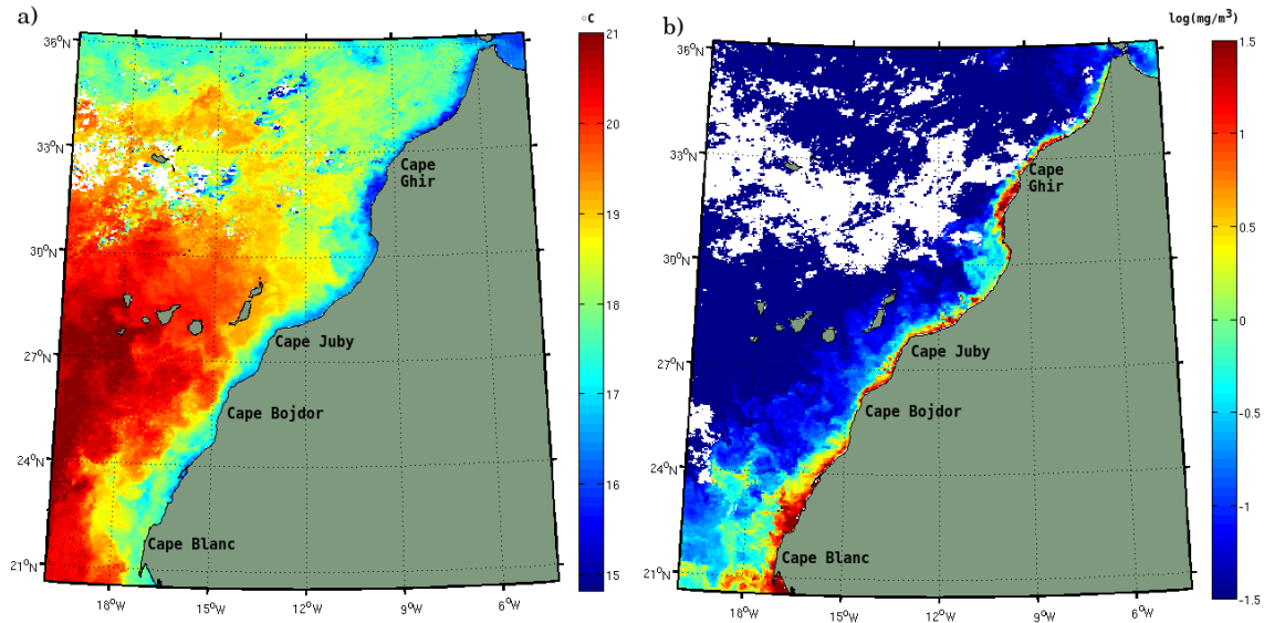
Figure 2-8: (a) 8-day SST image ( ^{\circ}\text{C} ), (b) \text{CHL}_a concentration ( \log(\text{mg}/\text{m}^3) ) image obtained on the first week of January 2007, showing typical upwelling scenario from physical and biological observations; similar oceanic structures appear in both images.
