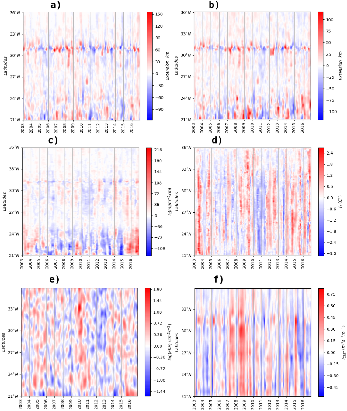
Figure 3-14: Space-time Hövmoller diagram presenting anomalies of: a) upwelling extension from SST, b) upwelling extension from CHL a , c) upwelling index ( I_c ) computed as the CHL a average multiplied by its extension, d) upwelling intensity I_T , e) eddy kinetic energy ( \text{cm}^2\text{s}^{-2} ) estimated from geostrophic velocities derived from satellite-derived sea level anomalies, f) Cross-shore Ekman Transport ( I_{CSET} ), over the 2003-2016 archive period.
