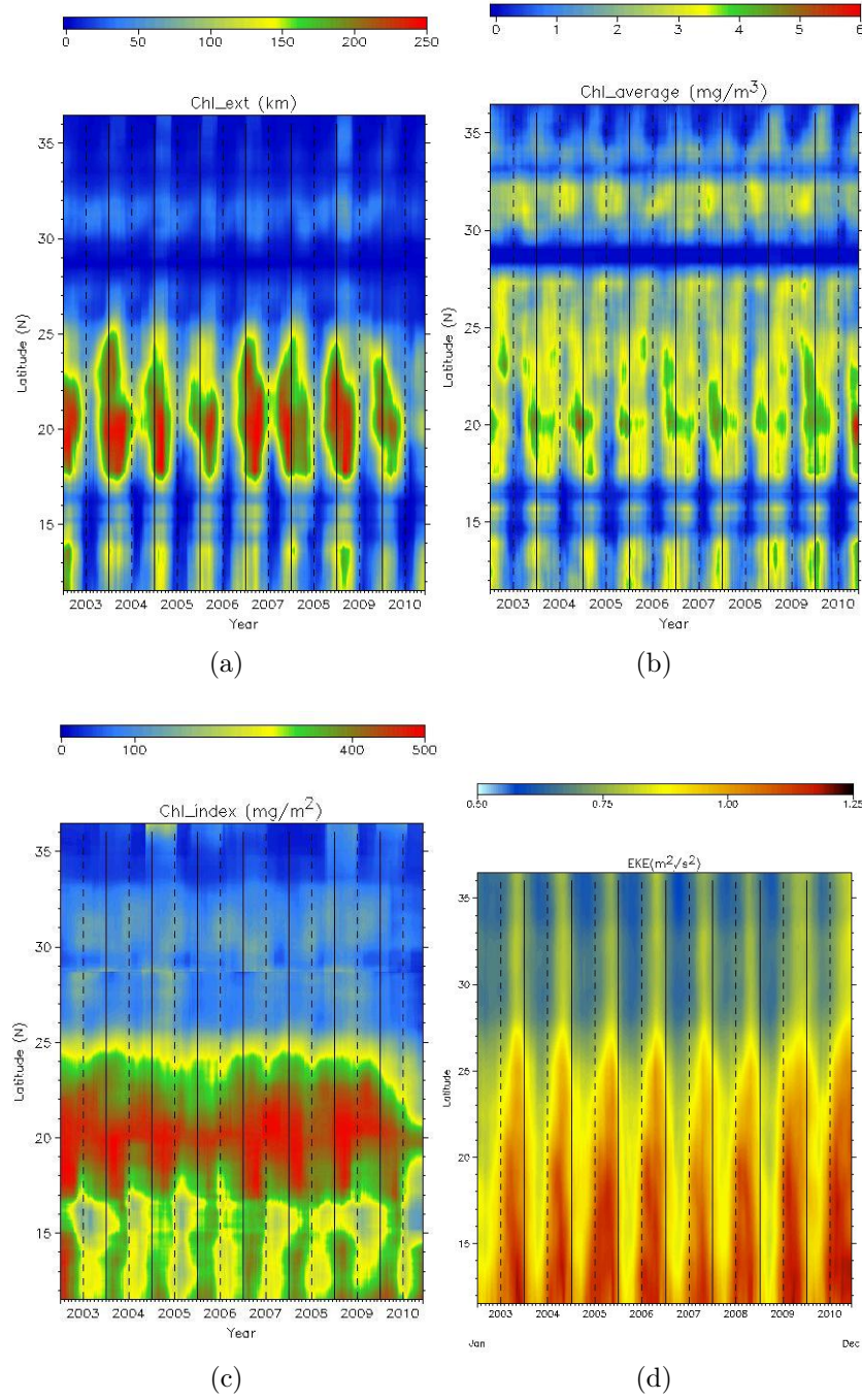
Figure 5-2: Space-time Hovmöller plot of the seasonal and interannual variability a) Upwelling extension ( Chl_{ext} ) calculated as 0.5mg \times m^{-3} limit, b) Chlorophyll averaged over the Upwelling area ( Chl_{avg} ), c) Upwelling index ( Chl_i ) computed as the chlorophyll average multiplied by its extension, d) the eddy kinetic energy (EKE) calculated for the period of time between [2003-2010].
