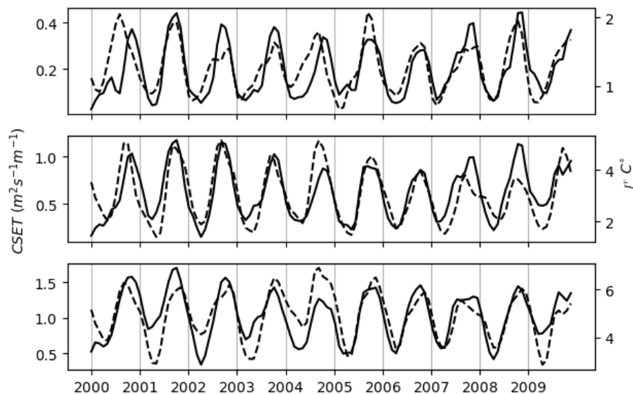
Figure 3-5: Comparative seasonal and interannual variability of the I^r (dotted lines) and the I_{CSET} from the Quikscat wind (plain lines) of the three characteristic areas previously identified (a)North, b)Central, d)South).
