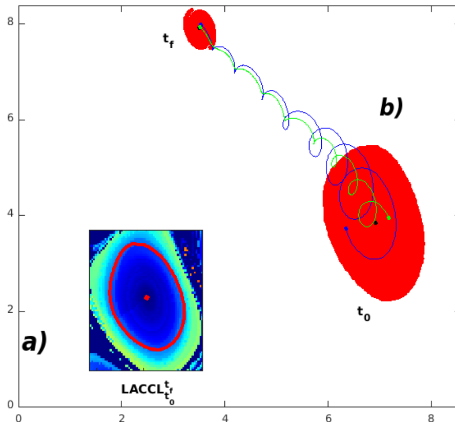
Figure 6-14: a) Coherent vortex and its center at time t_0 extracted using definition.1 with the \mathcal{LACCL}_{t_0}^{t_f}(\mathbf{x}_0) map shown in background. b) Its initial and final positions under Lagrangian advection. (See the supplemental movie M6 for the complete advection sequence of this vortices.).
