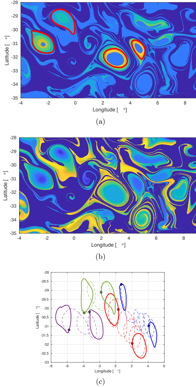
Figure 7-7: a) Coherent eddies at time t_0 extracted using definition.1 with the \bar{\xi} map shown in background, with \xi \mapsto |\mathcal{LTF}^\xi(\mathbf{x}_0)|^2 . b) The mean-average magnitude |\overline{\mathcal{LTF}^\xi(\mathbf{x}_0)}| highlighting areas of spinning movement. c) Their initial and final positions under Lagrangian advection as well as different particles initialized within their boundaries and their trajectories in Dashed line. (See the supplemental movie M8 for the complete advection sequence of these vortices.)
