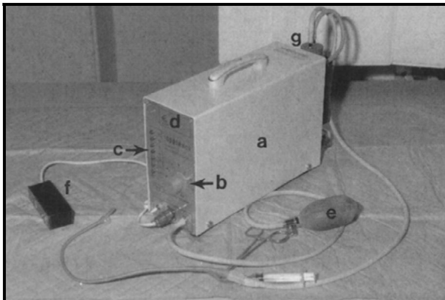
Figure 18:appareil d'insufflation [64]
